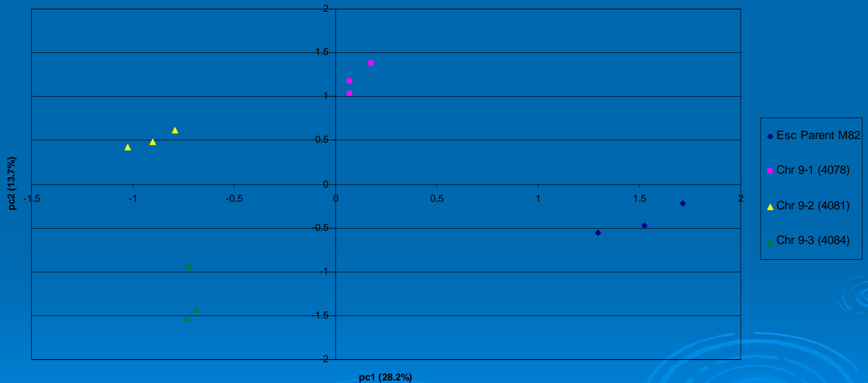
PCA Analysis of Chromosome 9
