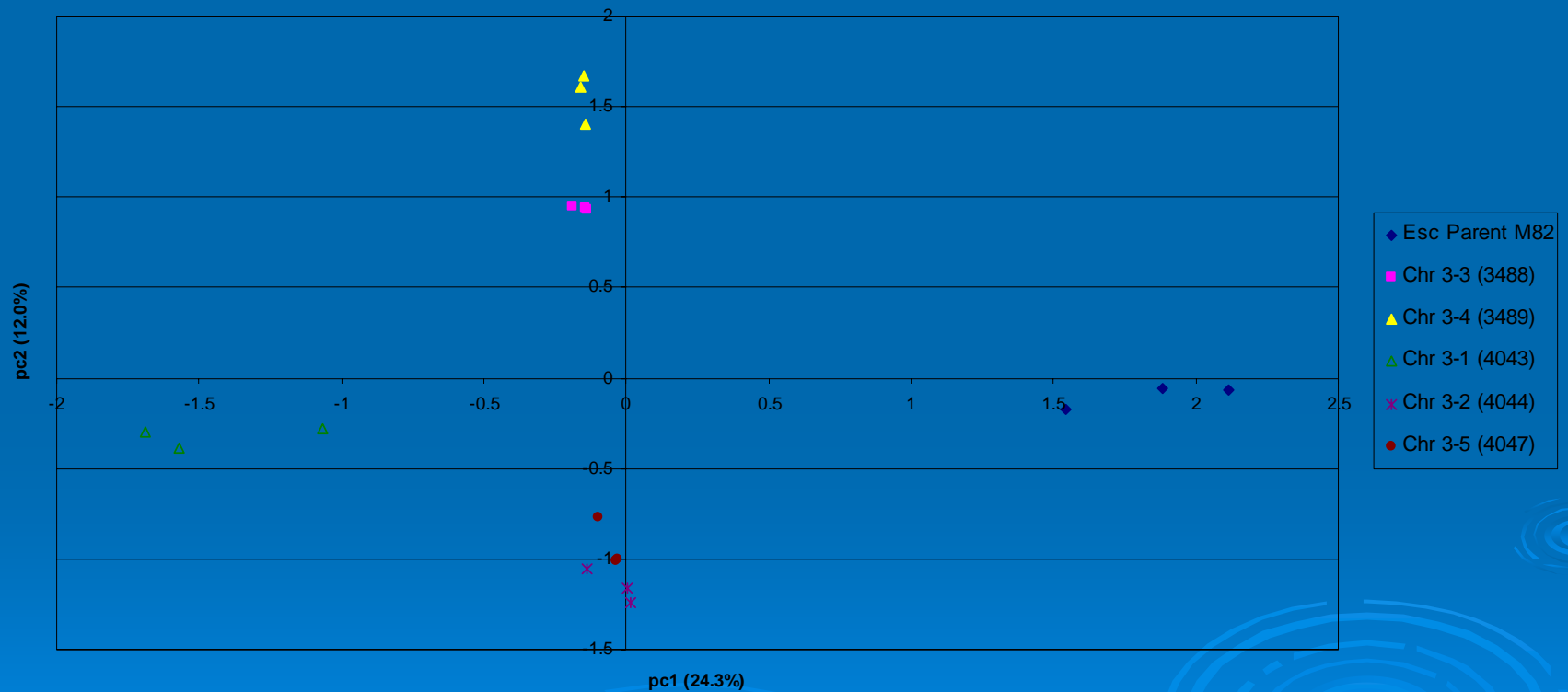
PCA Analysis of Chromosome 3
