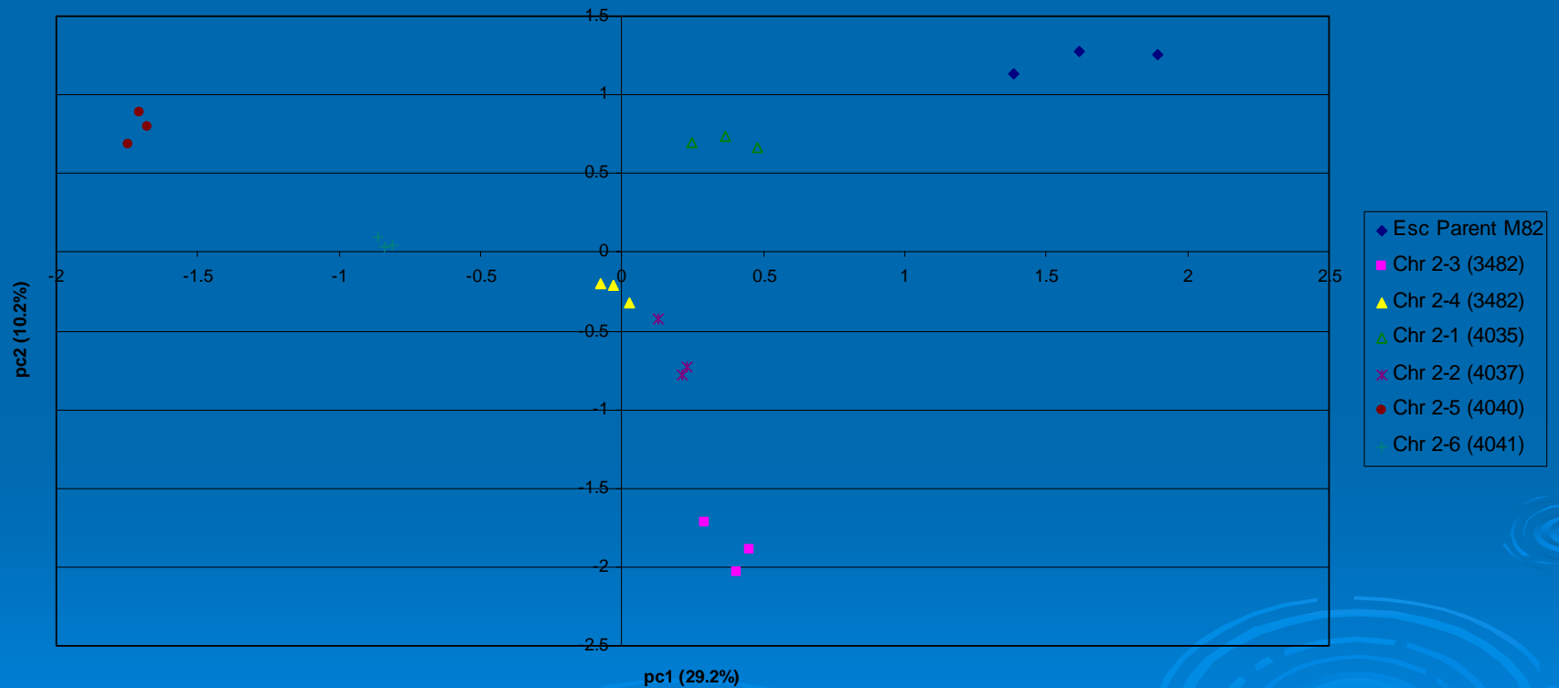
PCA Analysis of Chromosome 2
