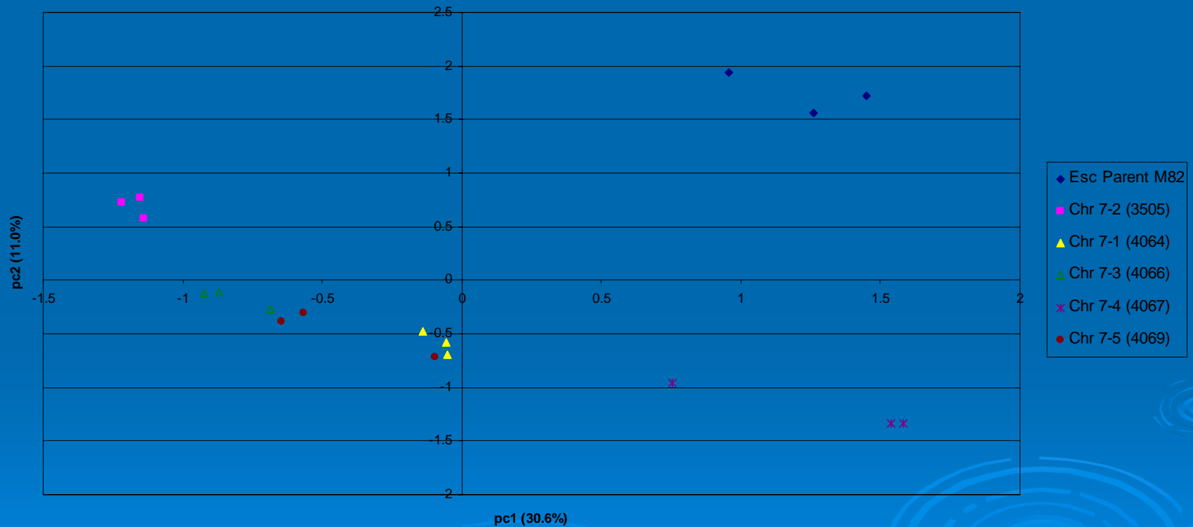
PCA Analysis of Chromosome 7
