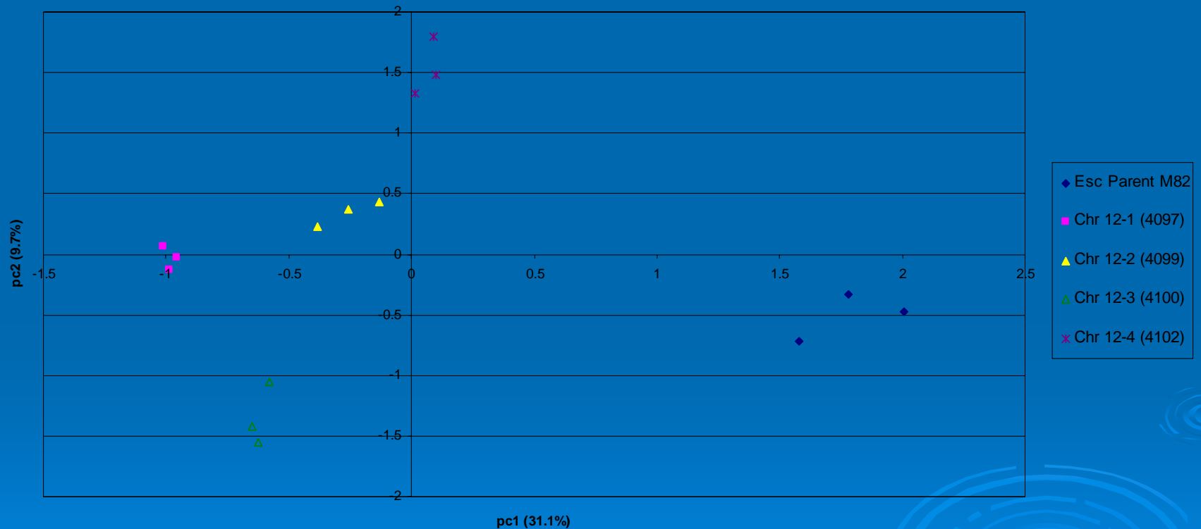
PCA Analysis of Chromosome 12
