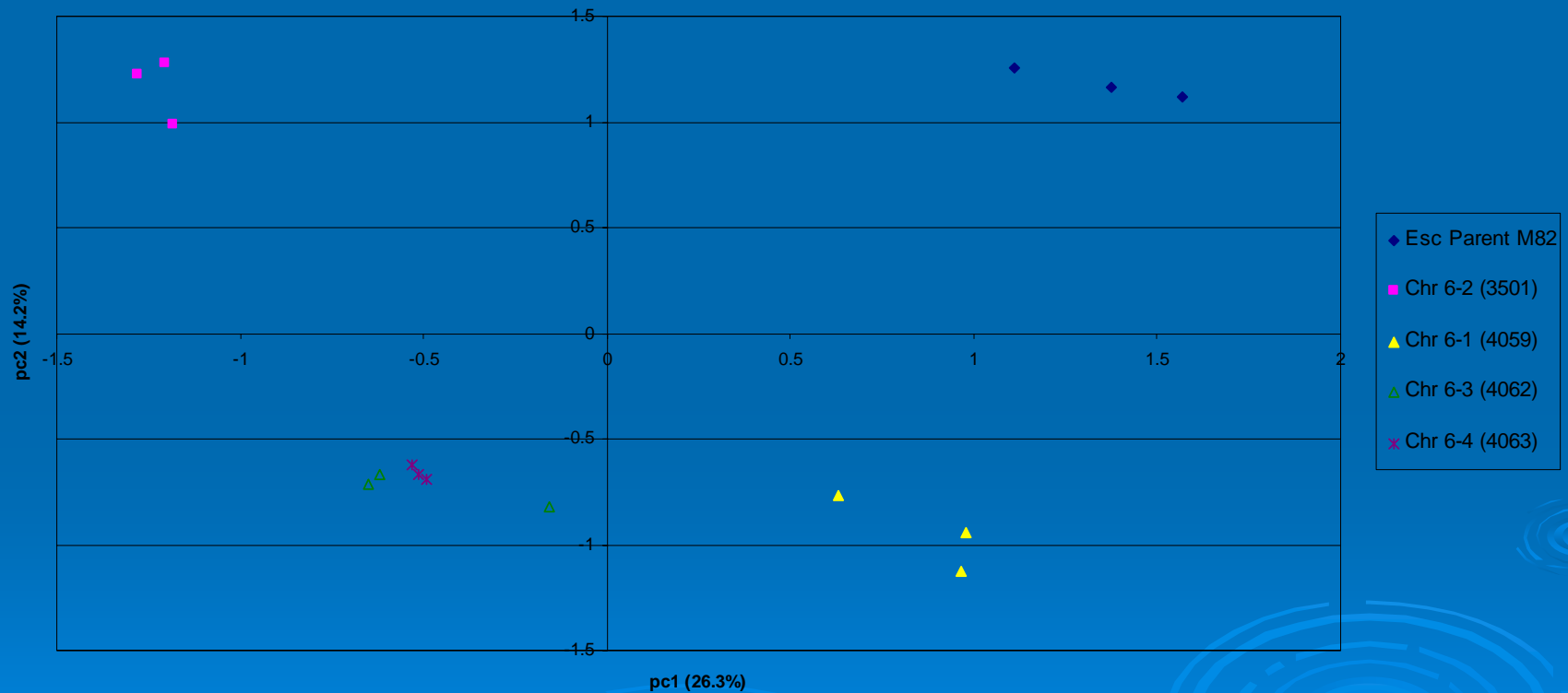
PCA Analysis of Chromosome 6
