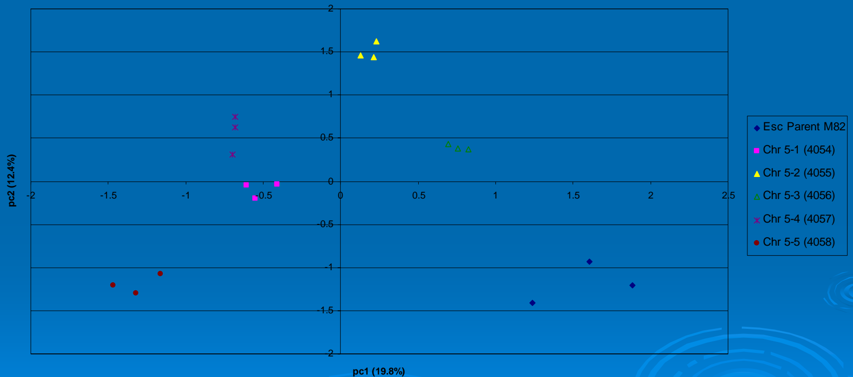
PCA Analysis of Chromosome 5
