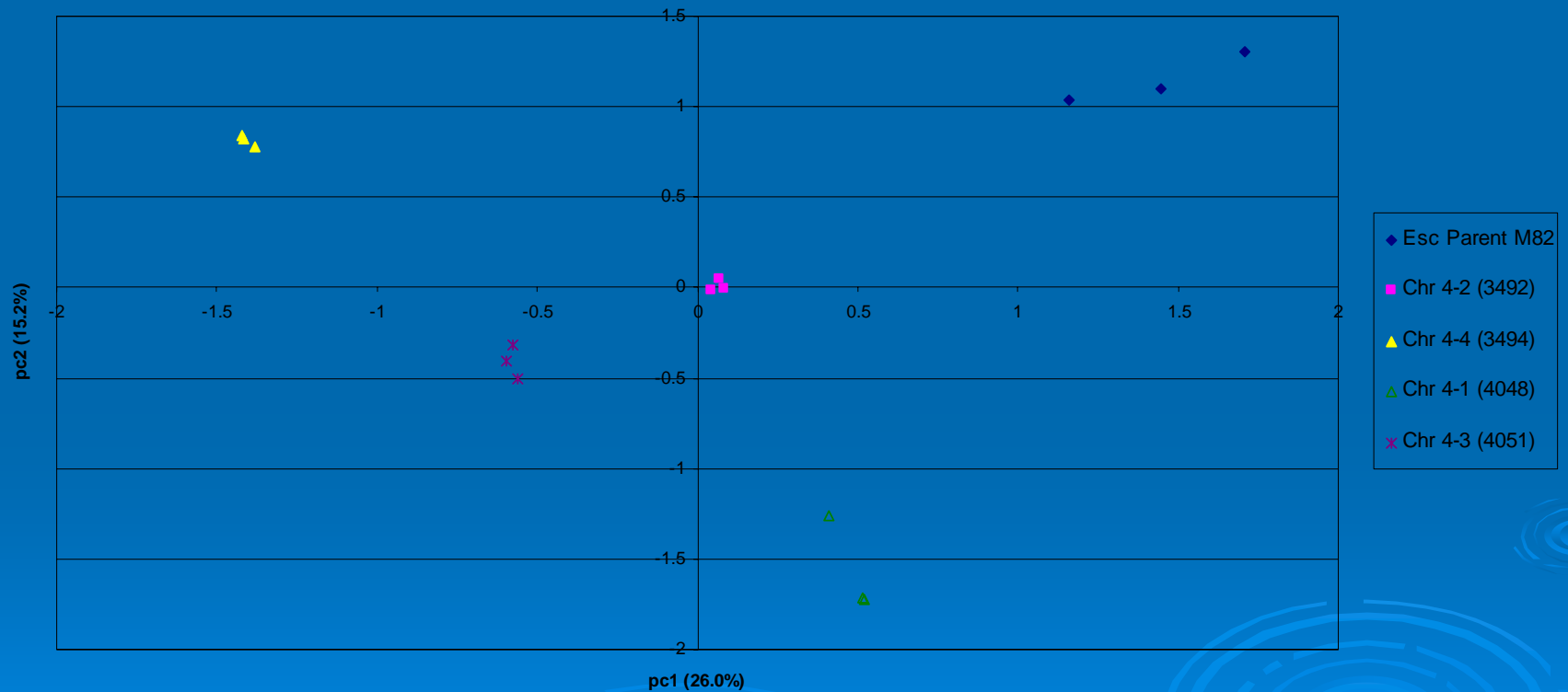
PCA Analysis of Chromosome 4
