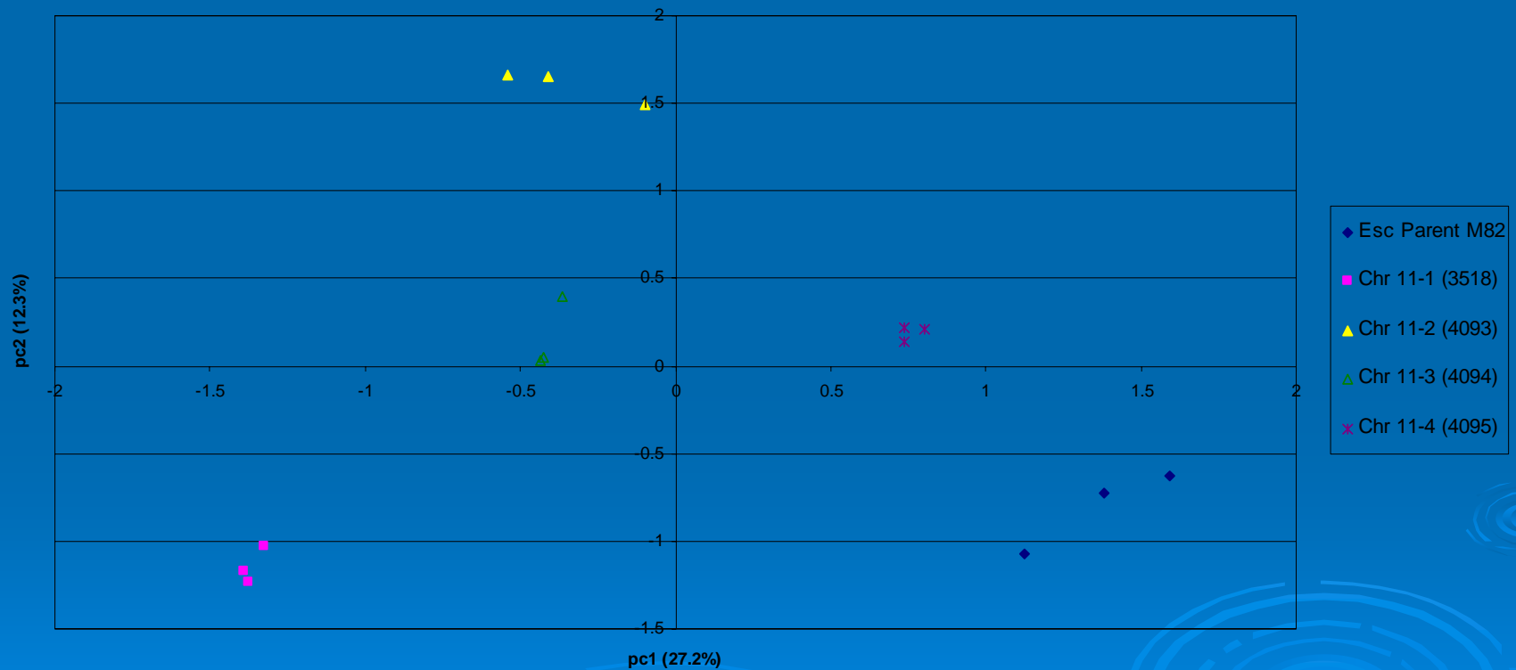
PCA Analysis of Chromosome 11
