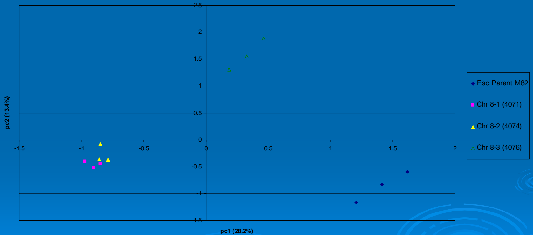
PCA Analysis of Chromosome 8
