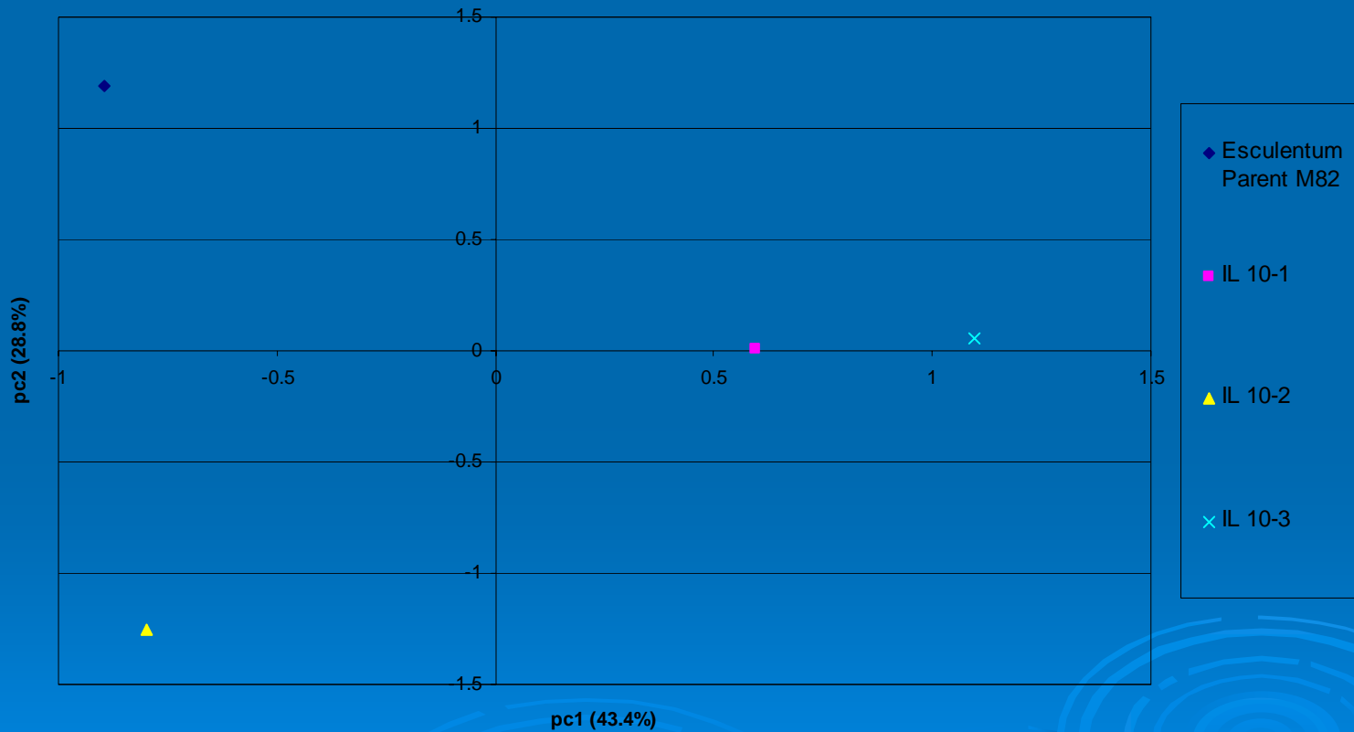
PCA Analysis of Chromosome 10 in Positive MS Mode
