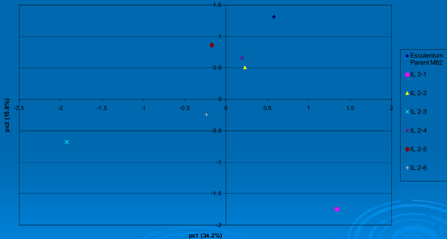
PCA Analysis of Chromosome 2 in Positive MS Mode
