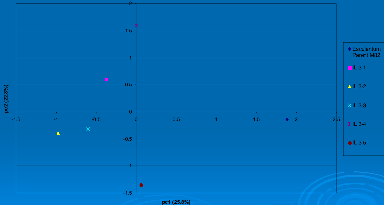
PCA Analysis of Chromosome 3 in Positive MS Mode
