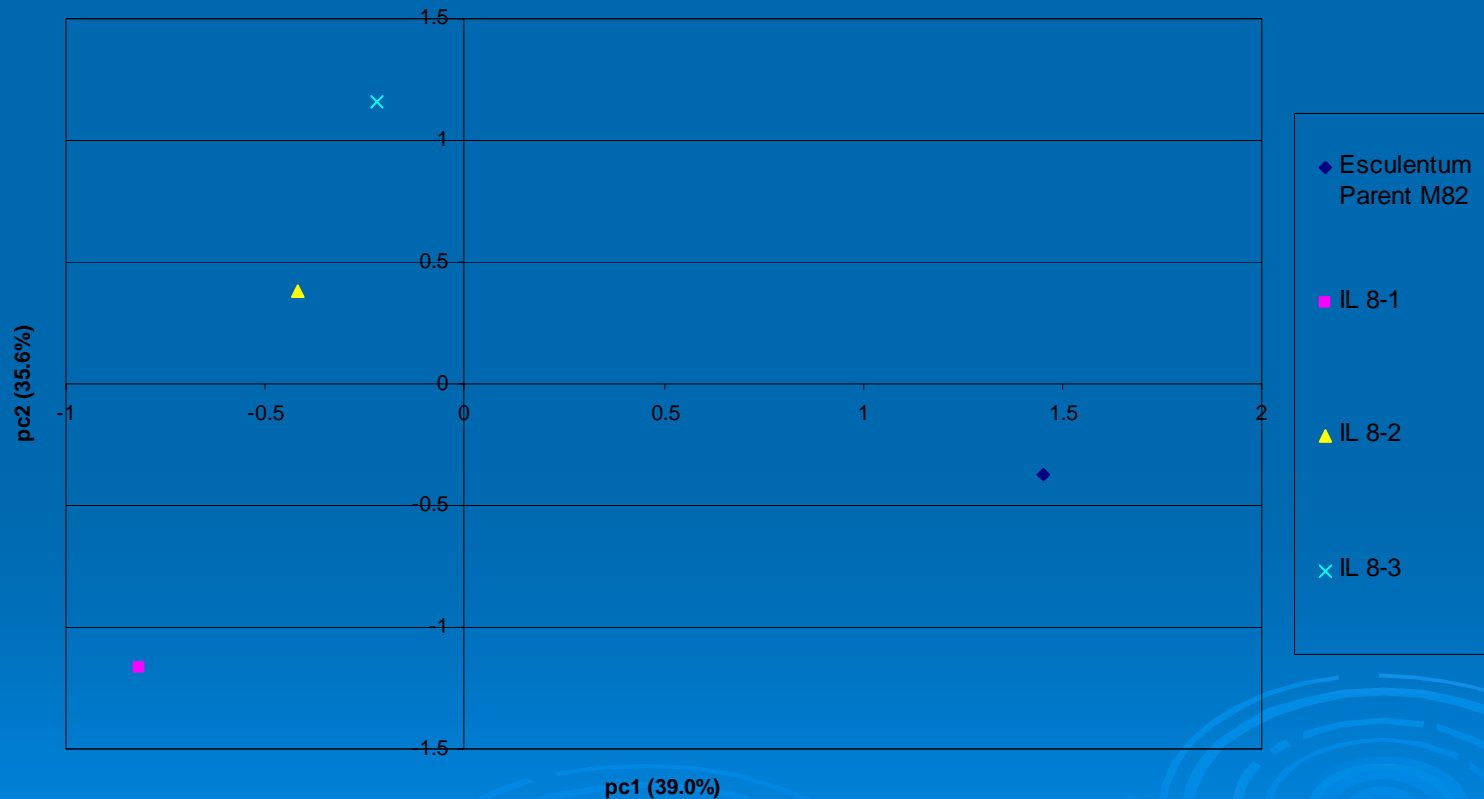
PCA Analysis of Chromosome 8 in Positive MS Mode
