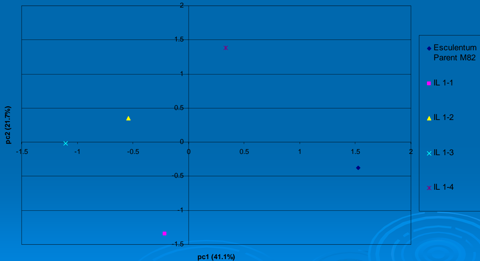
PCA Analysis of Chromosome 1 in Positive MS Mode
