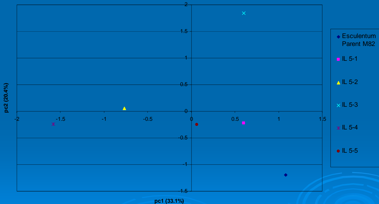
PCA Analysis of Chromosome 5 in Positive MS Mode
