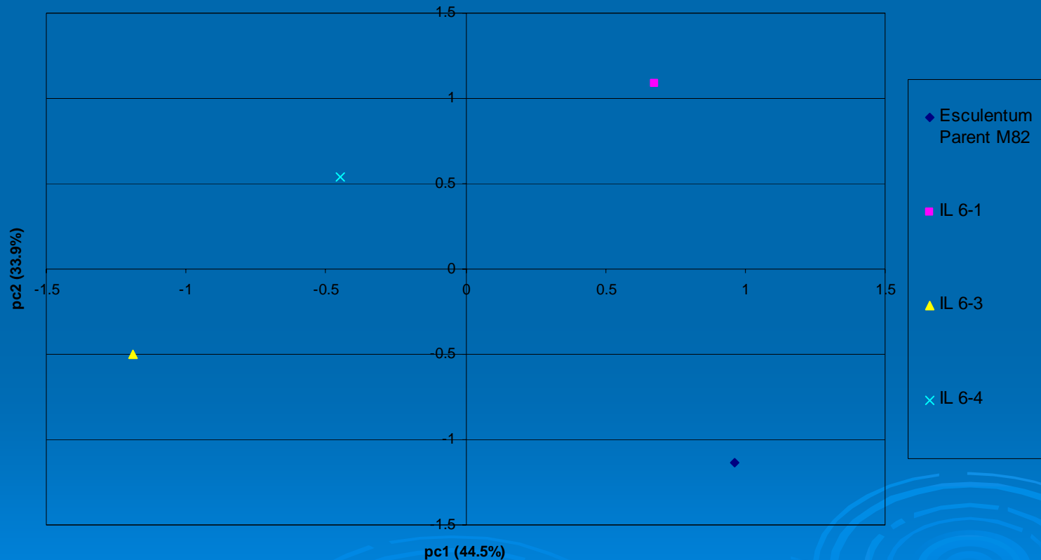
PCA Analysis of Chromosome 6 in Positive MS Mode
