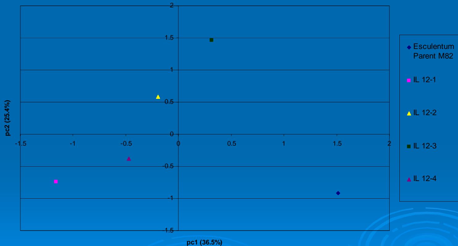
PCA Analysis of Chromosome 12 in Positive MS Mode
