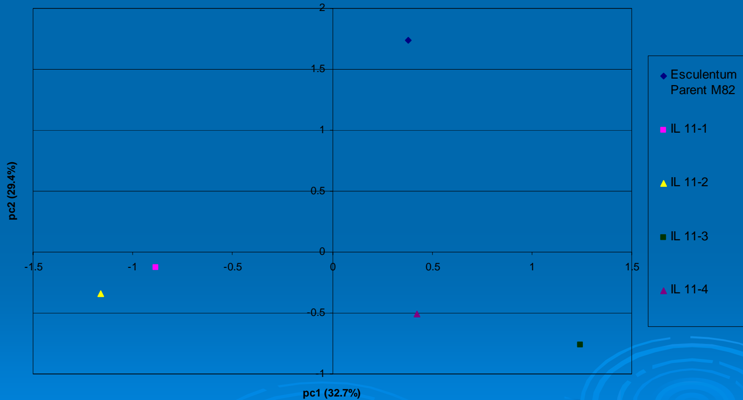
PCA Analysis of Chromosome 11 in Positive MS Mode
