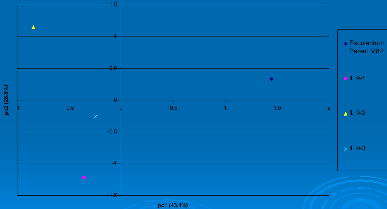
PCA Analysis of Chromosome 9 in Positive MS Mode
