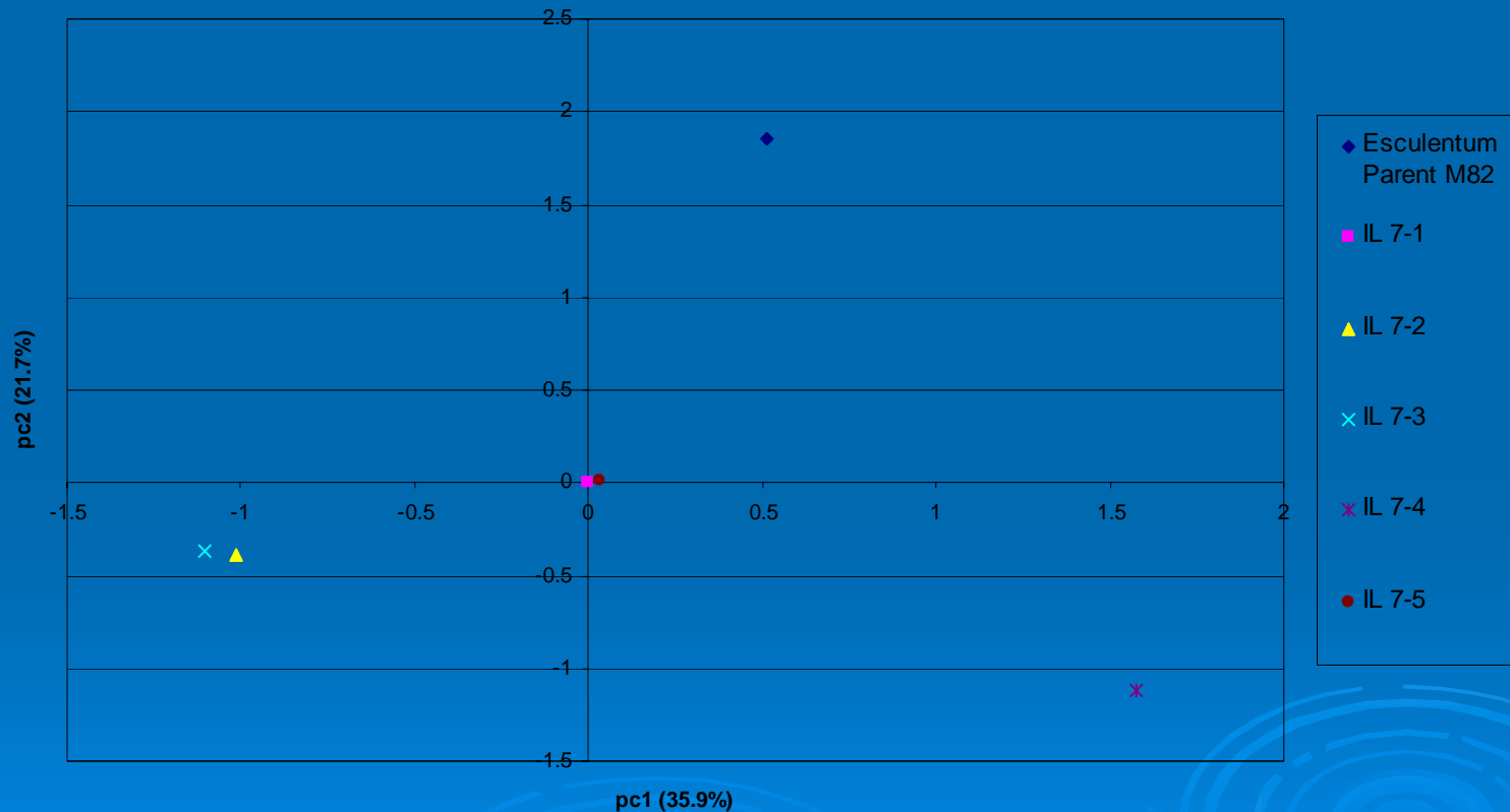
PCA Analysis of Chromosome 7 in Positive MS Mode
