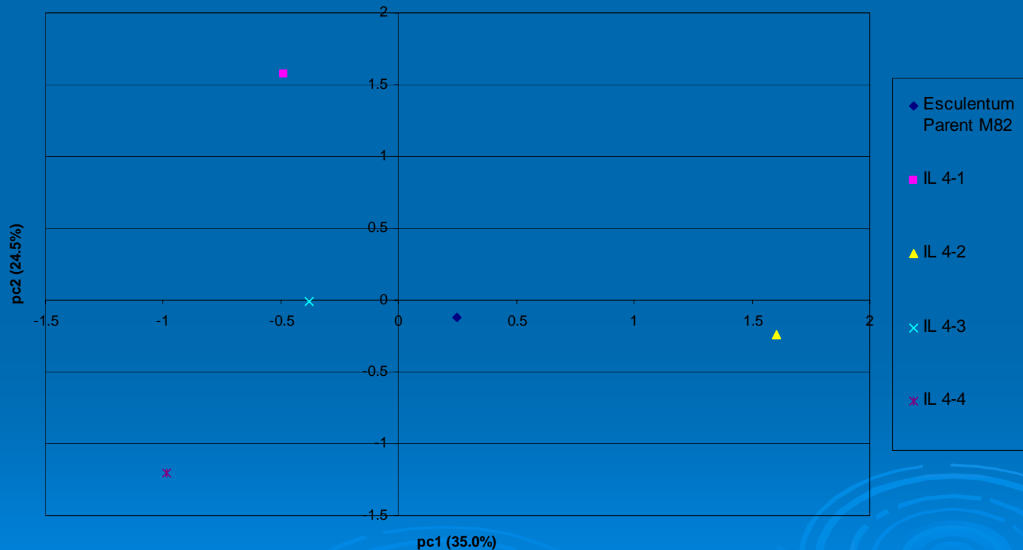
PCA Analysis of Chromosome 4 in Positive MS Mode
